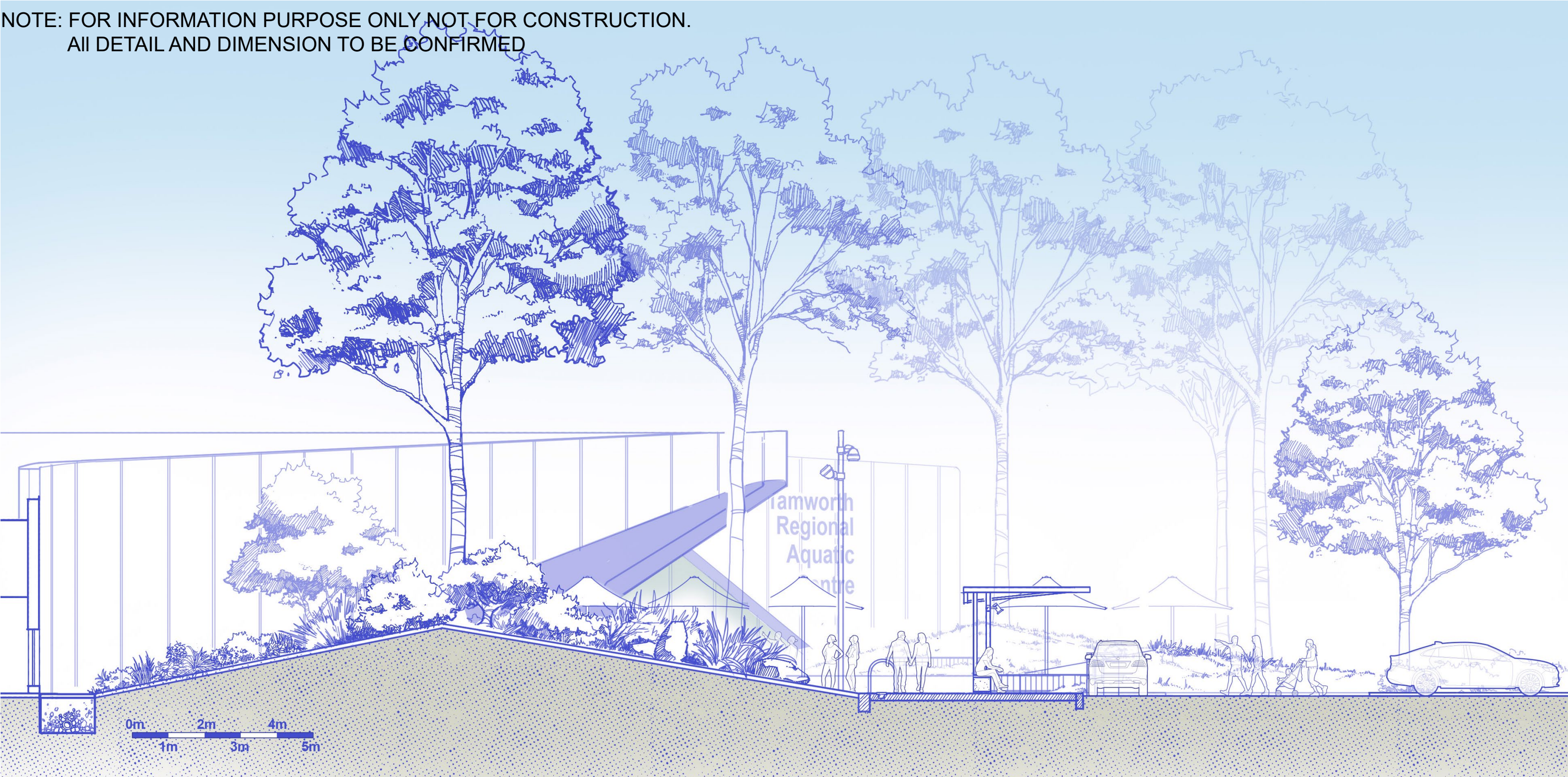
SECTION 1-1 1:100 IN A1
